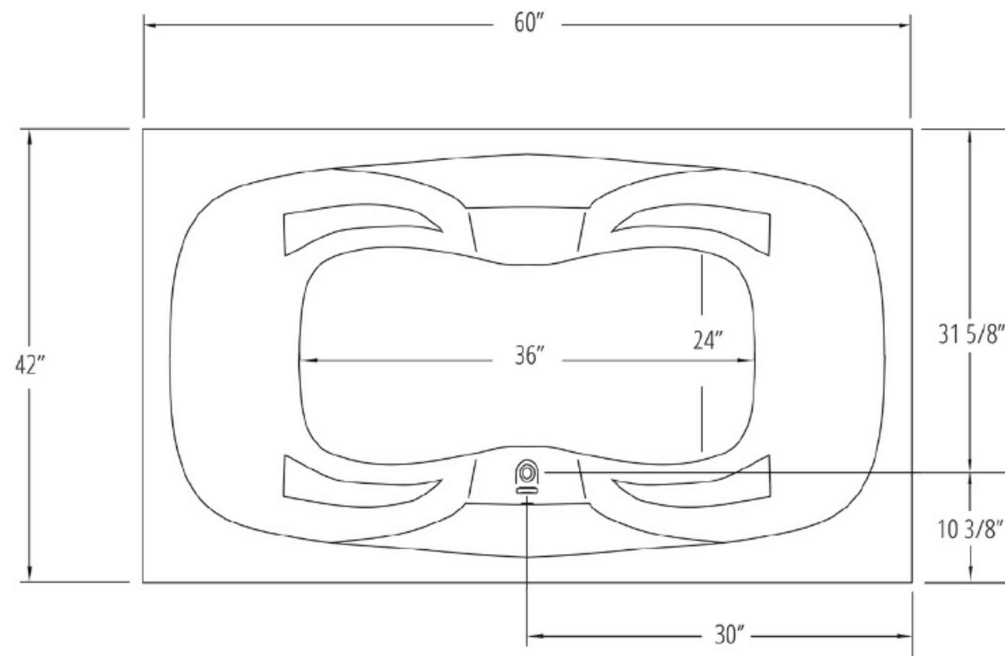
6 Jet Bathtub
