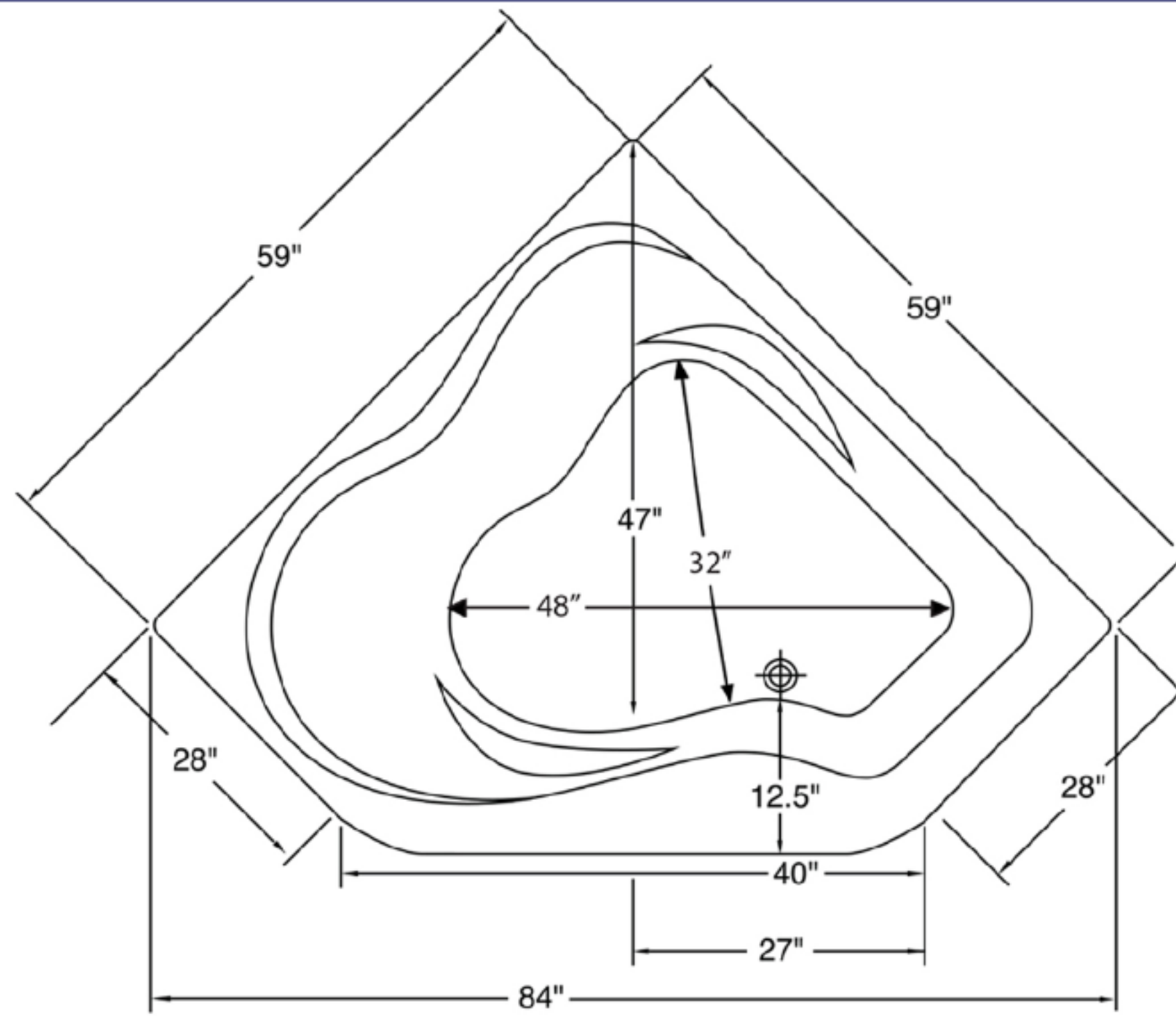
6 Jet Bathtub
