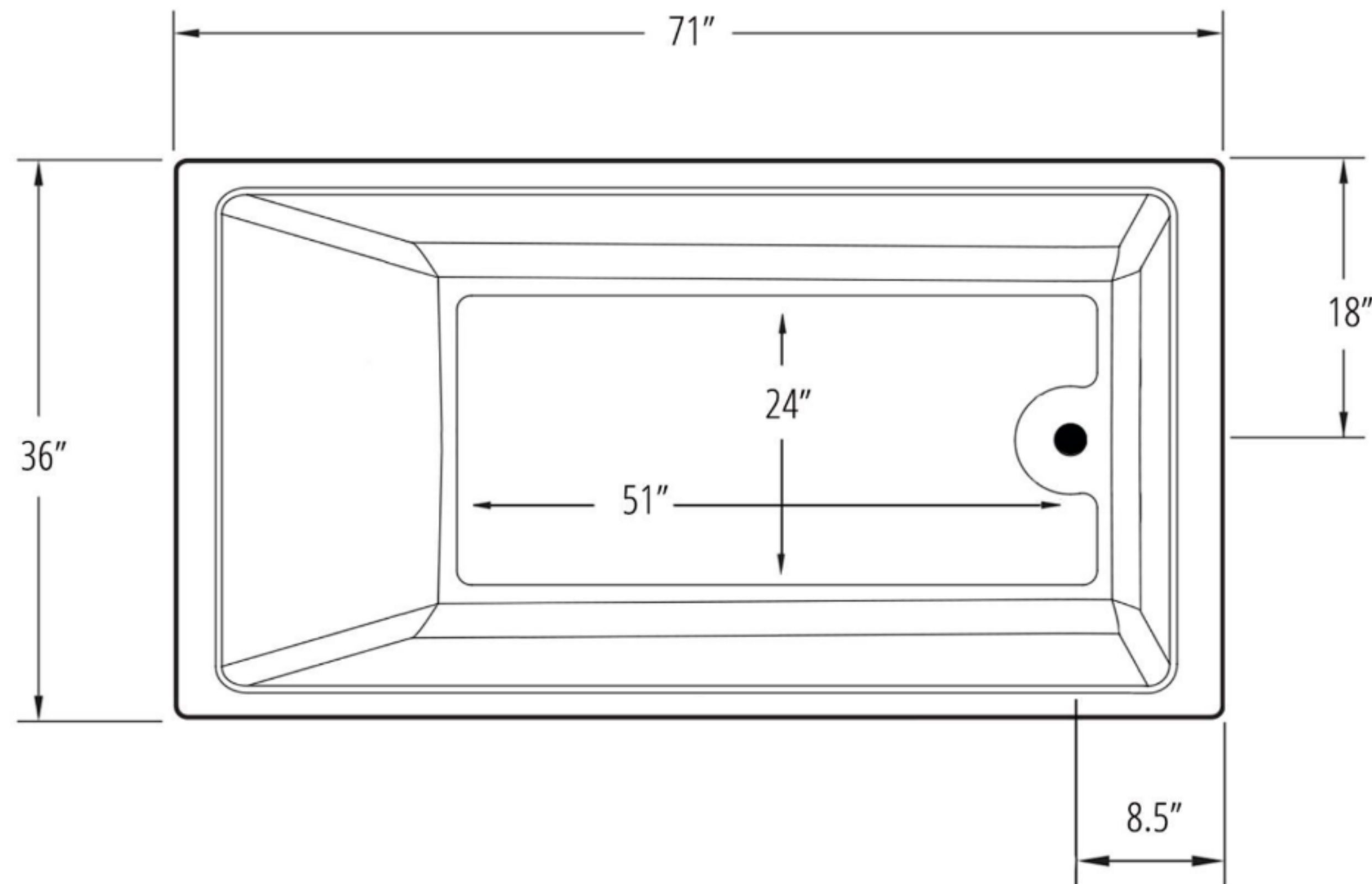
6 Jet Bathtub
