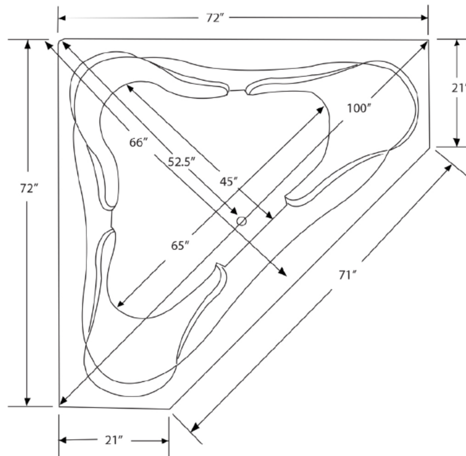
6 Jet Bathtub
